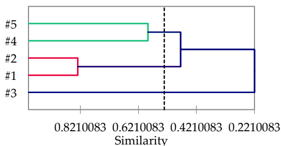
Figure 3. Dendrogram based on hierarchical cluster analysis of Purshia tridentata var. tridentata essential oil compositions.
