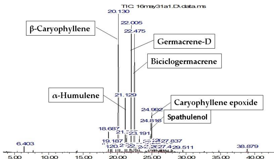
Figure 1. GC chromatogram (HP-5 column) and representative compounds of leaves of Vernonia gracilis Kunth.
