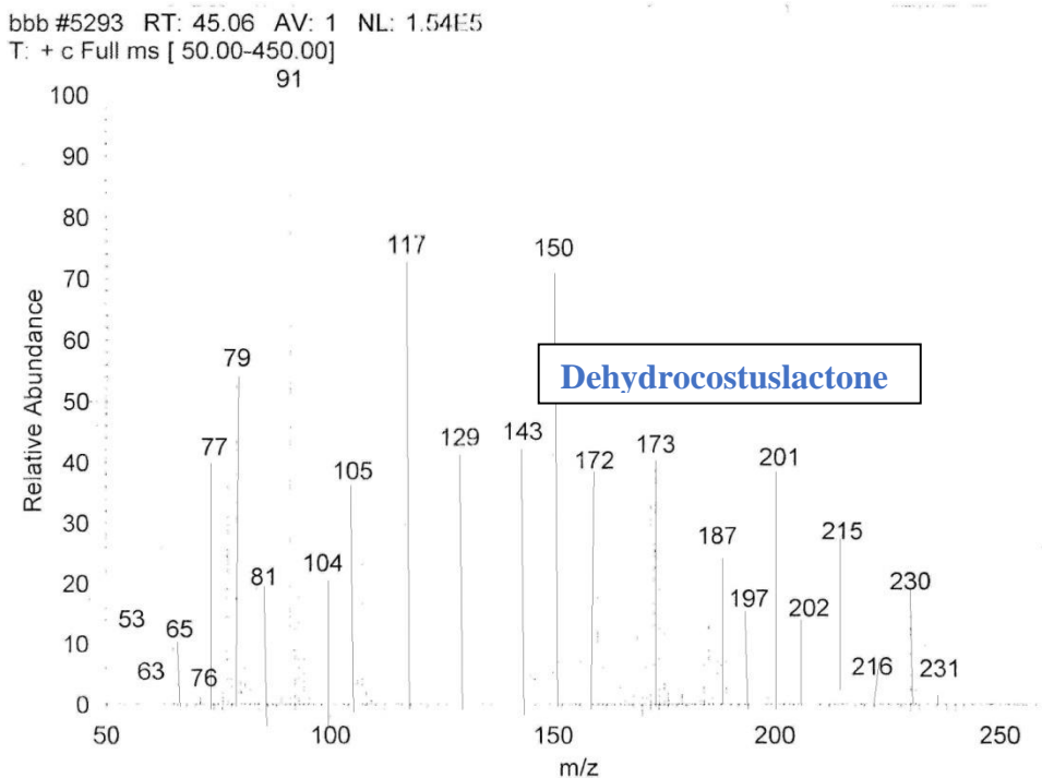
Figure S2. Mass spectrum of Dehydrocostuslactone (SL-02)
