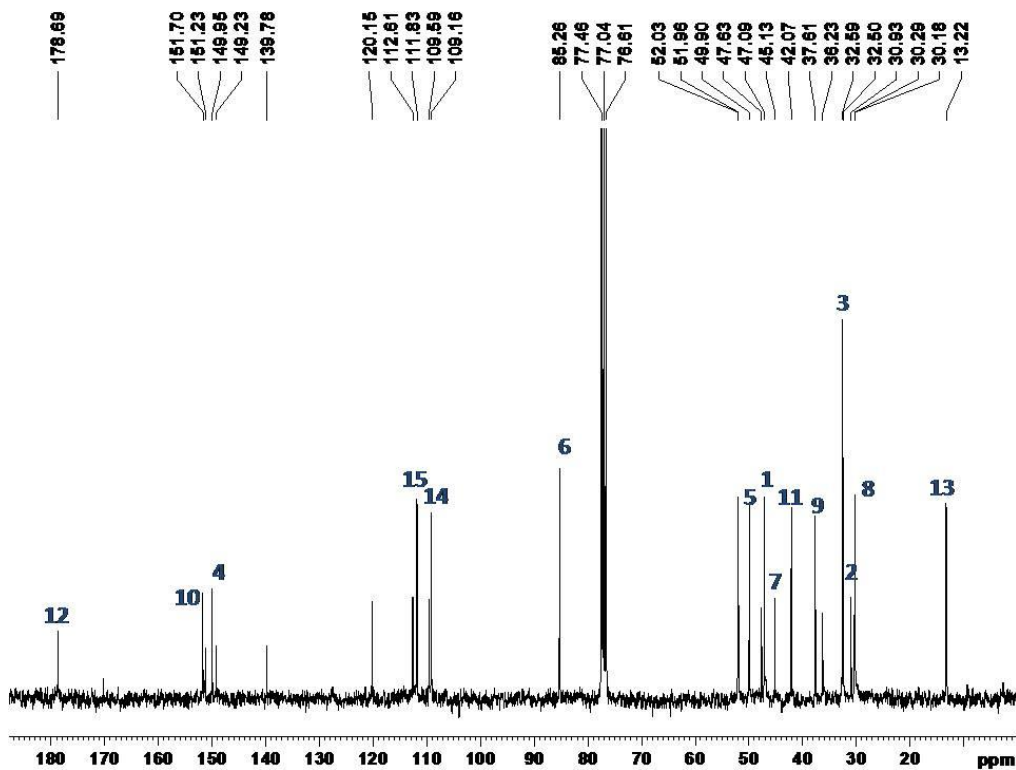
Figure S4. 13 C NMR spectrum of Dihydrodehydrocostuslactone (SL-01)
