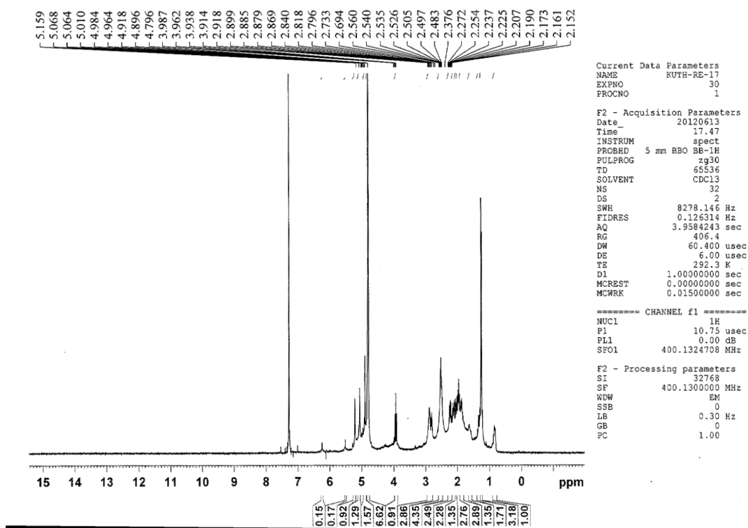
Figure S5. 1 H NMR spectrum of Dehydrocostuslactone (SL-02)
