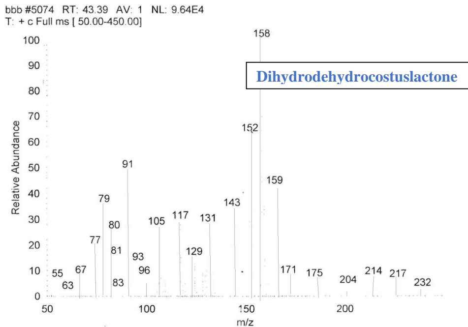
Figure S1. Mass spectrum of Dihydrodehydrocostuslactone (SL-01)
