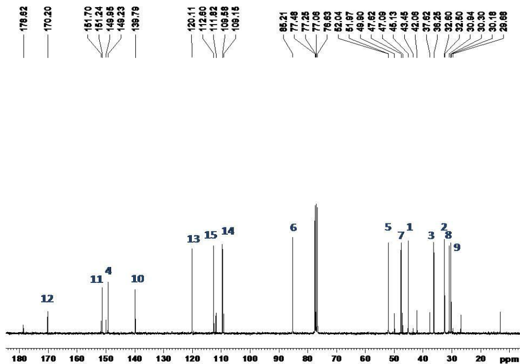
Figure S6. 13 C NMR spectrum of Dehydrocostuslactone (SL-02)
