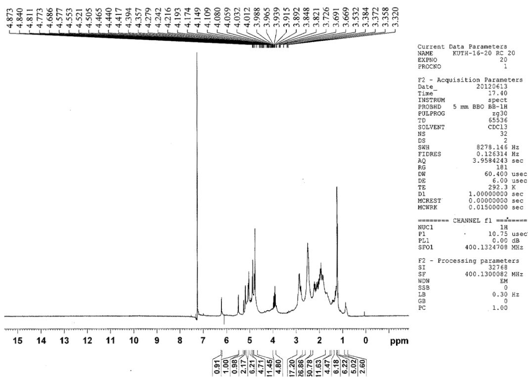
Figure S3. 1 H NMR spectrum of Dihydrodehydrocostuslactone (SL-01)
